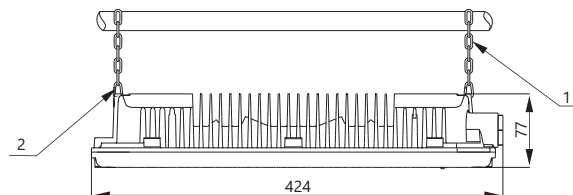
Chain type mounting(standard)
